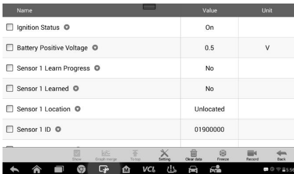
Figure 4-14 Sample Live Data Screen
