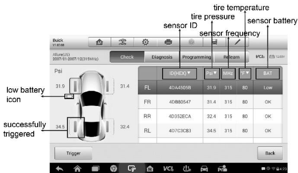
Figure 4-8 Sample Check Screen 2
